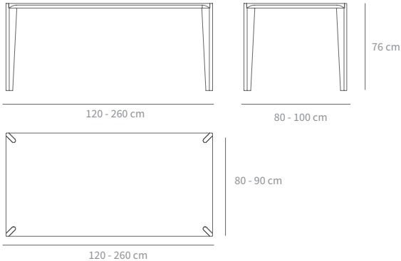
Technical drawing of the Hanny table showing top and side views with dimensions.
