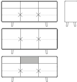
1. H 90 W 200 D 47 CM WITH 3 DOORS + 3 DRAWERS 2. H 90 W 200 D 47 CM WITH 3 DOORS 3. H 90 W 200 D 47 CM WITH 3 DOORS + 2 DRAWERS + 1 OPEN COMP.
