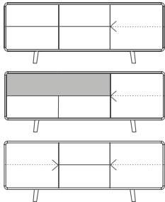
1. H 75 W 200 D 47 CM WITH 1 DOOR + 4 DRAWERS 2. H 75 W 200 D 47 CM WITH 1 DOOR + 2 DRAWERS + 1 OPEN PART 3. H 75 W 200 D 47 CM WITH 2 DOORS + 2 DRAWERS
