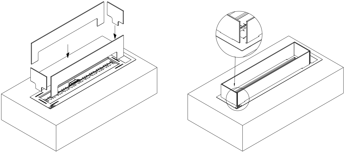
Fig. 4 – Glass installation
