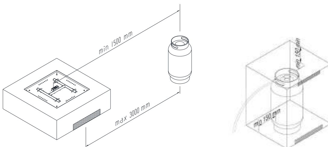
Fig 5 – Gas cylinder distance
