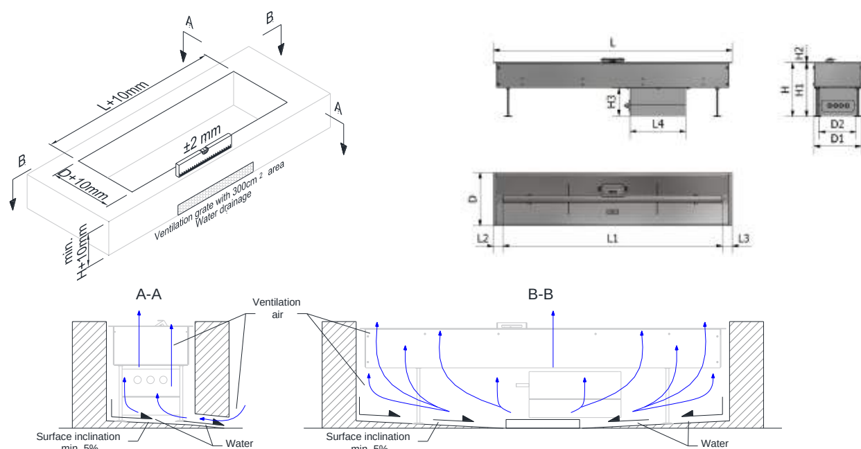
Fig. 4 – Cavity measures for units above 1500mm
