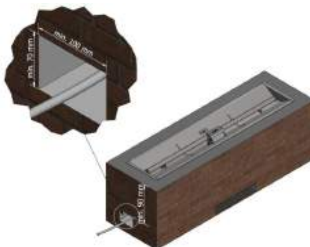
Fig. 7 – Installation for LPG type unit
