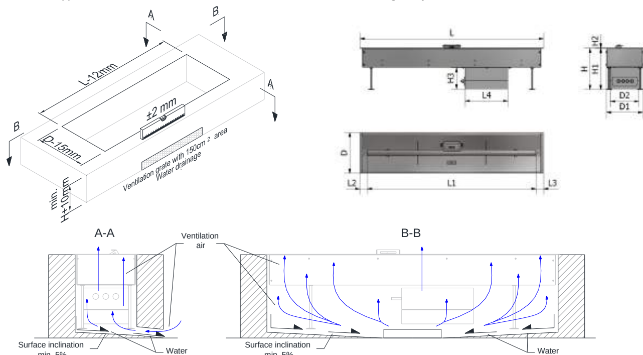
Fig. 3 – Cavity measures for units up to 1500mm
