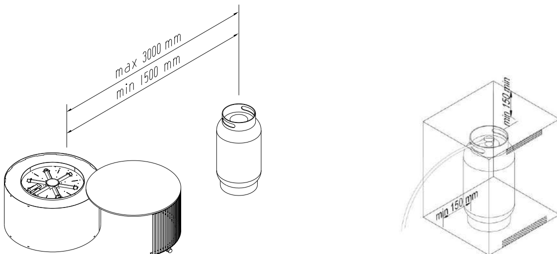
Fig. 4 – Gas cylinder distance
