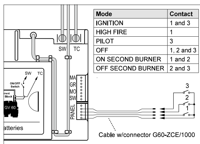
Figure 1: Wiring diagram and the operation sequence.
