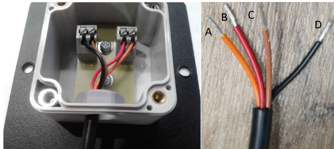
Wallswitch interior
